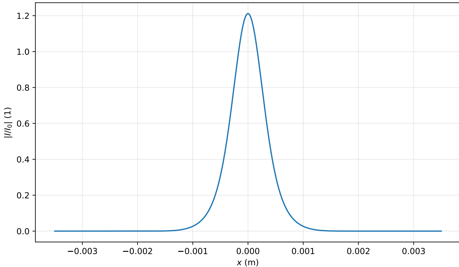
Intensity profile I(x, y = 0, z = 1.194m)/I_0 , P_{in}=0.7P_{cr} , artificial time
